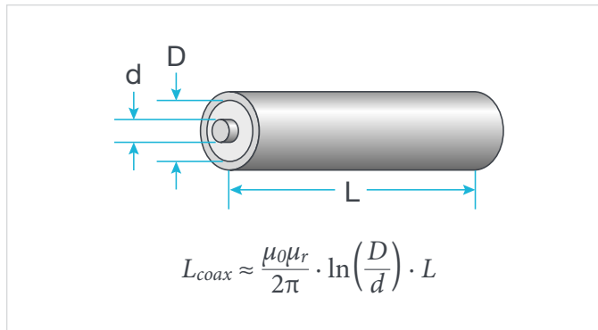
Figure 4. Coaxial cable inductance
