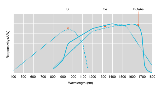
Figure 8. The choice of detector depends largely on the wavelength of light involved.
