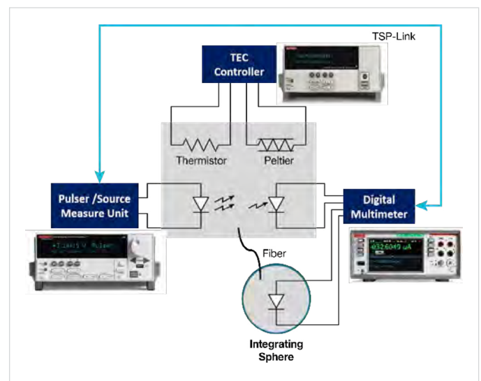
Figure 10. Typical LIV Test Setup for a Laser Diode Module. The same instrumentation can be applied for testing VCSELs. The 2601B-PULSE is used to source current pulses at 10 A @ 10 V at 10 \mu s to the device under test and monitor the light output with a digital multi-meter while the Thermal Electric Cooler (TEC) is controlling the module temperature.
