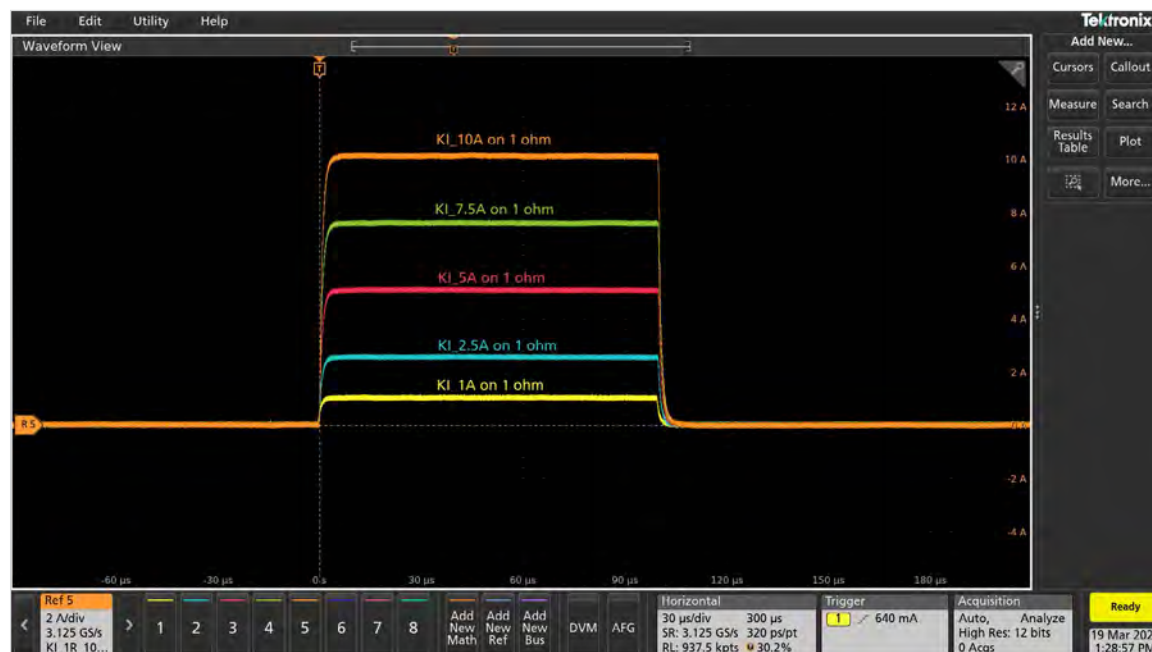
Figure 3: Amplitude sweep at 1 A, 2.5 A, 5 A, 7.5 A, and 10 A on a VCSEL
