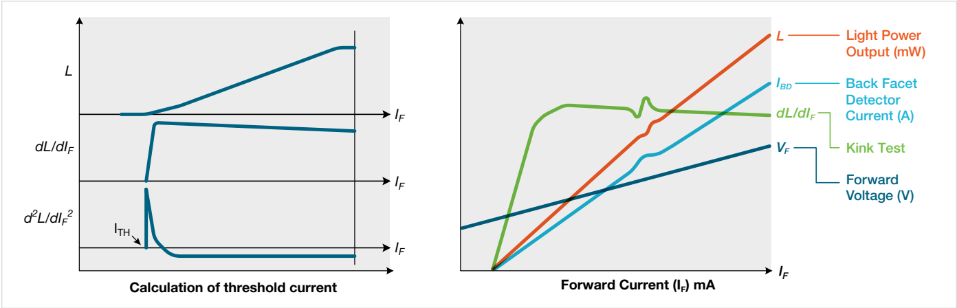
Figure 1: LIV curves
