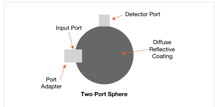
Figure 9. An integrating sphere solves the problem of coupling instrumentation to the output of the laser diode.
