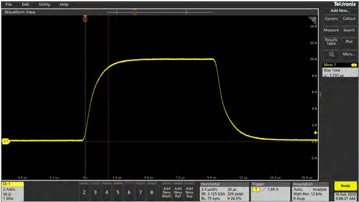
Figure 2: 10 A, 10 μs current pulse with 1.7 μs rise time
